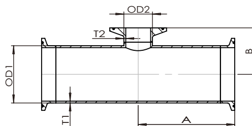
卡式短切异径三通 Clamp Joint: Short-Outlet Reducing Tee 316L
