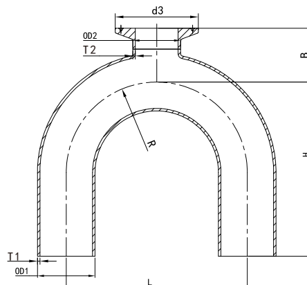
DIN11865 U型弯单卡三通 C系列 304L Automatic Weld: Clamp Joint 180° Return-Bend Reducing Tee
