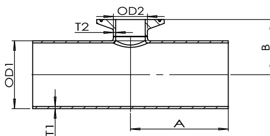
单卡短切异径三通 Automatic Weld: Short-Outlet Clamp, Joint Reducing Tee 316L
