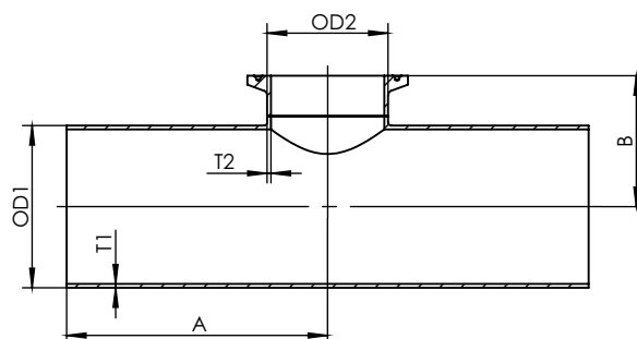
单卡短切异径三通 Automatic Weld: Short-Outlet Clamp, Joint Reducing Tee 316L
