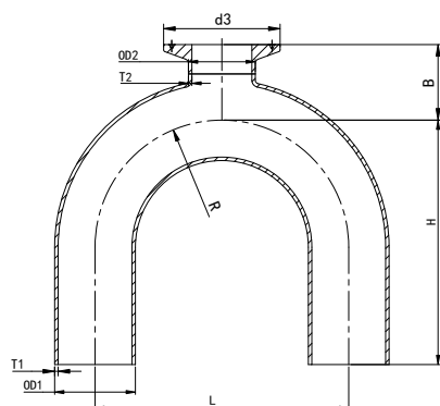
3A U型弯单卡三通 异径 316L Automatic Weld: Clamp Joint 180°Return-Bend Reducing Tee
