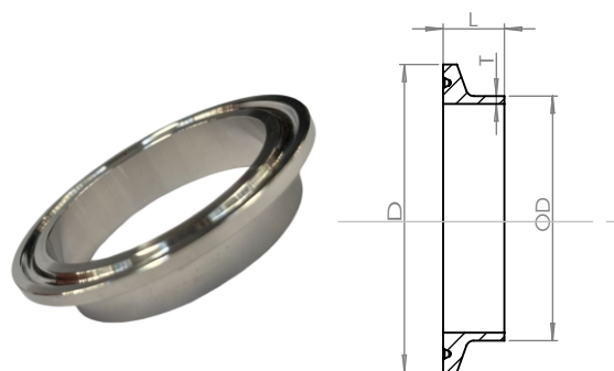
TYPE B
