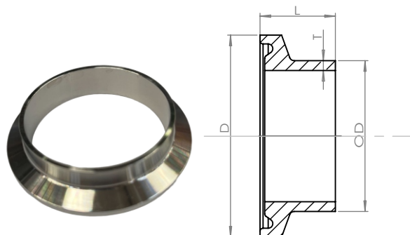
TYPE A
