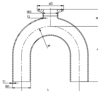
3A U型弯单卡三通 异径 304L Automatic Weld: Clamp Joint 180°Return-Bend Reducing Tee
