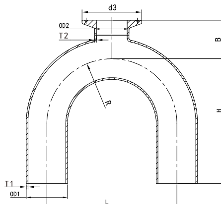
DIN11865 U型弯单卡三通 C系列 316L Automatic Weld: Clamp Joint 180° Return-Bend Reducing Tee
